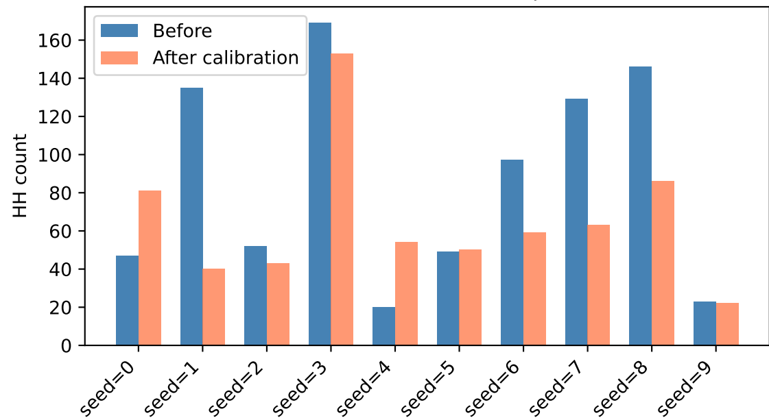
HH count: before vs after — ('compas', 'isotonic')
